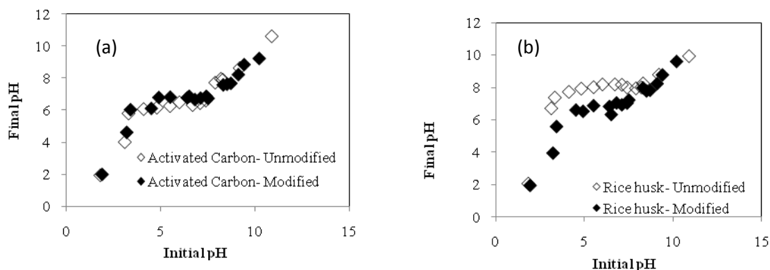
Figure 1: pHzpc of modified and unmodified materials. (a) Activated carbon (b) Rice husk ash
