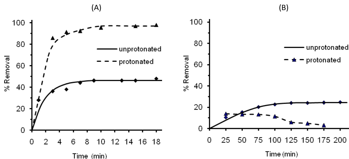
Figure 1. Percentage removal of (A) Cr(III) and (B) Cr(VI) by unprotonated and protonated dry C. caroliniana biosorbent at different shaking times (biosorbent dosage 2.0 g L -1 , initial metal ion concentration 5.0 mg L -1 , pH 5.0, temperature 25 °C, shaking speed 140 rpm).
