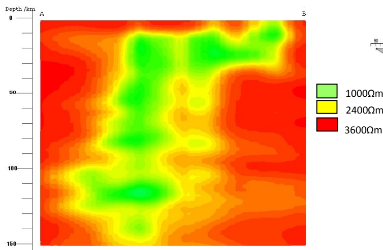
Fig. 1. Apparent resistivity profile of Mahapalassa traverse. Total length of the section (A-B) is 26kms.
