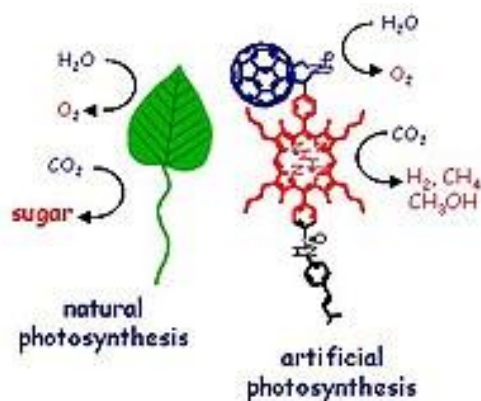
Schematic diagram of natural and artificial photosynthesis
