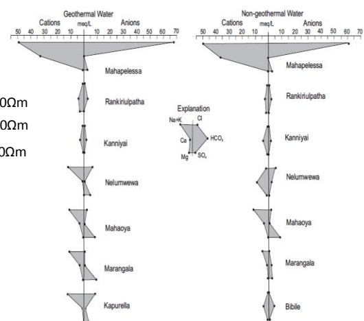
Fig.2. Comparison of chemical compositions of geothermal and non-geothermal waters.
