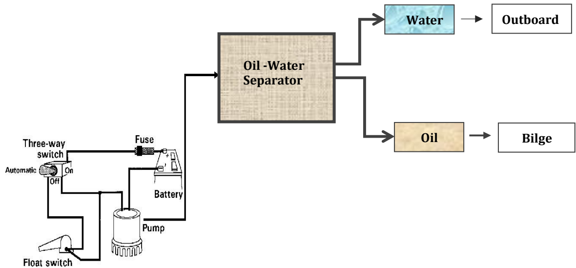
Newly designed bilge system
