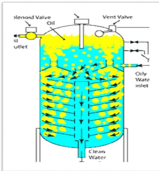
Oil water separator
