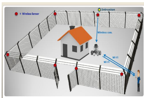
Security Robot sensor network
