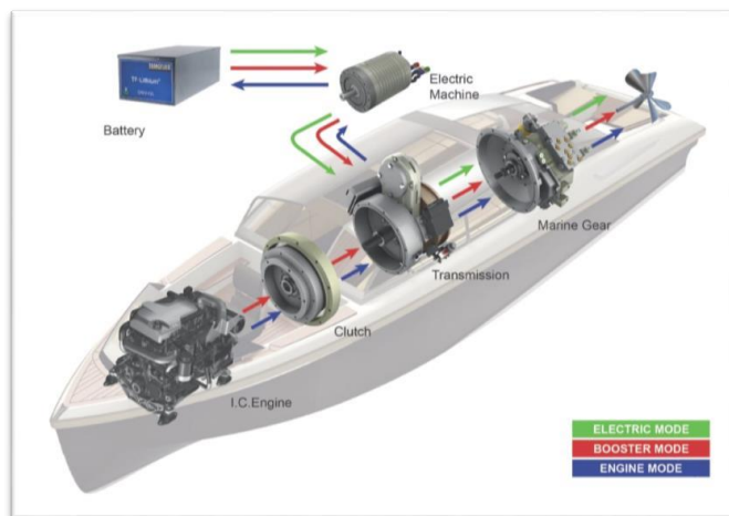
Marine Diesel Hybrid Engine
