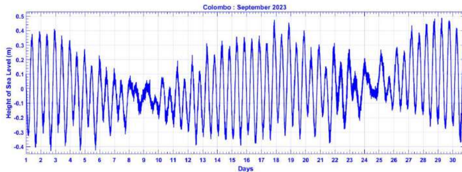
Figure 01: Sea level variation at Colombo
