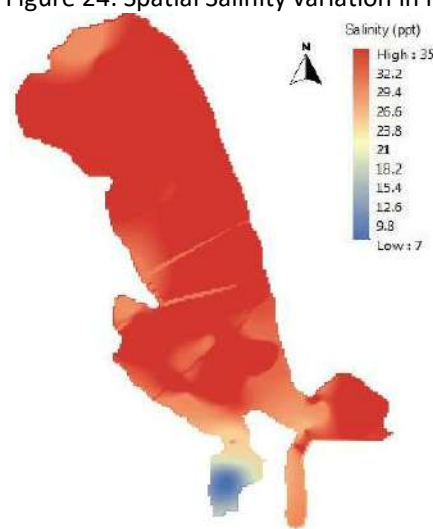
Figure 26: Spatial Salinity variation in October
